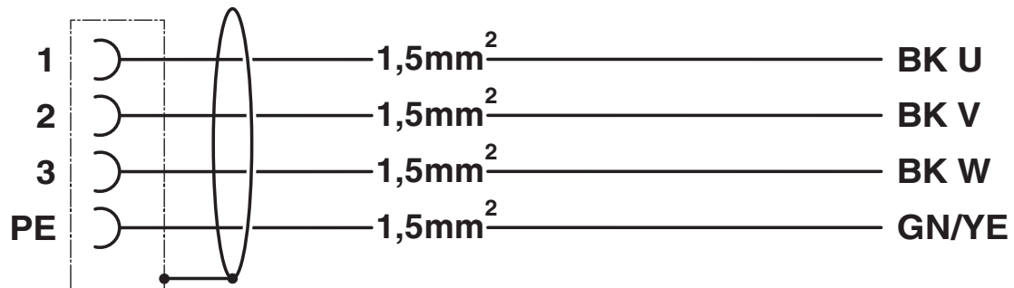
Circuit diagram
