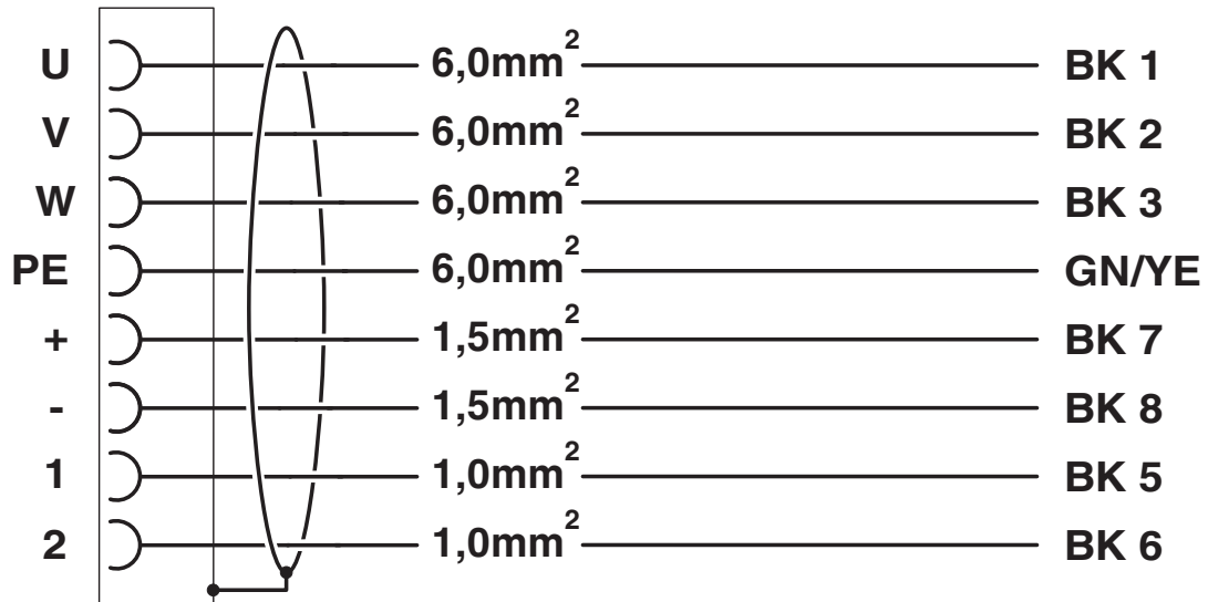
Circuit diagram
