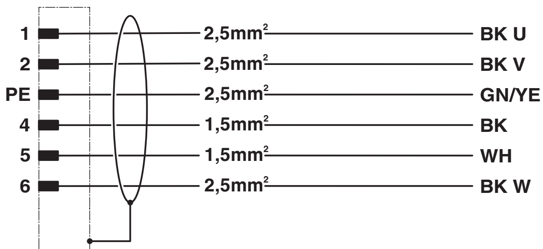
Circuit diagram
