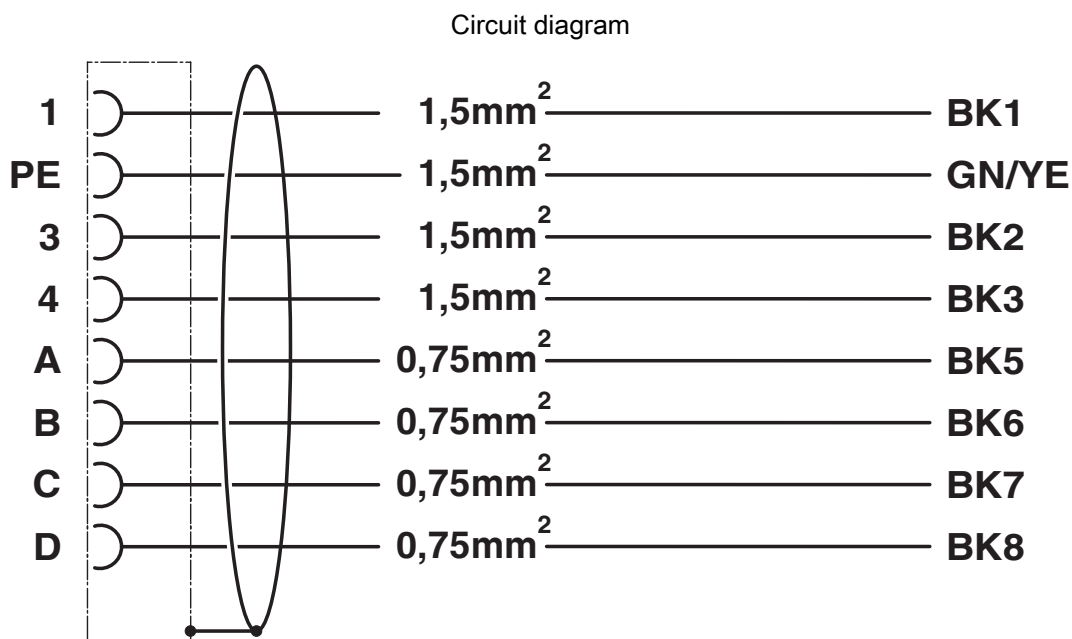
Connector pin assignment
