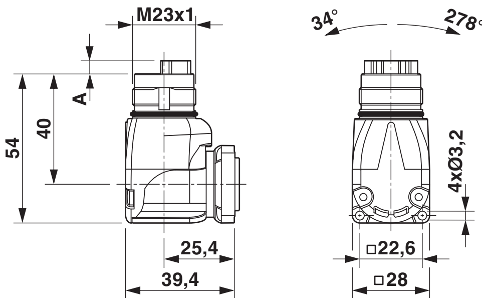
Dimensional drawing
