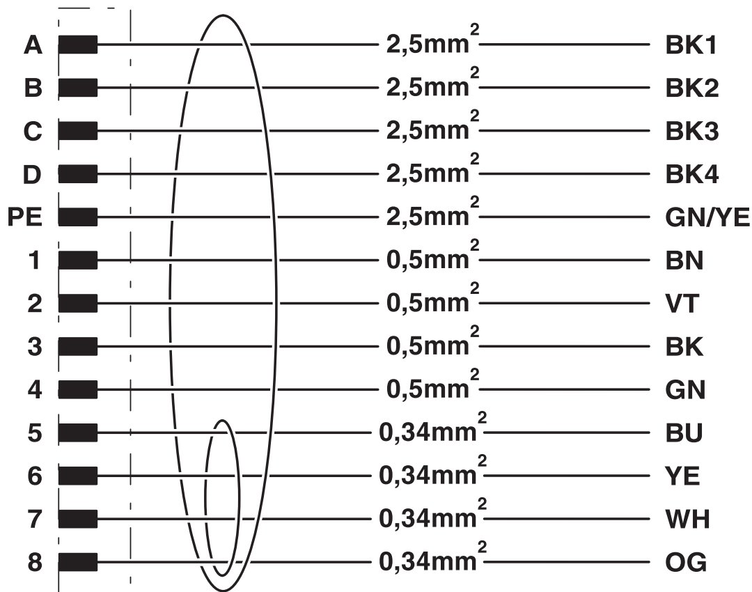
Circuit diagram
