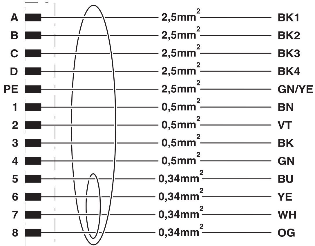
Circuit diagram
