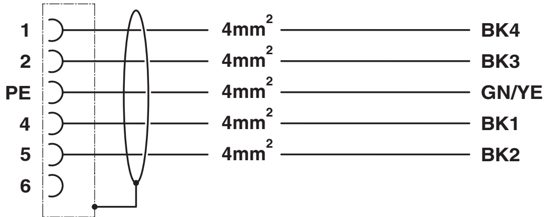
Circuit diagram
