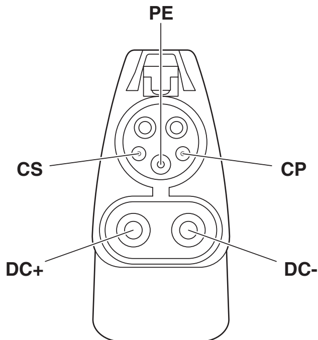
Connection diagram
