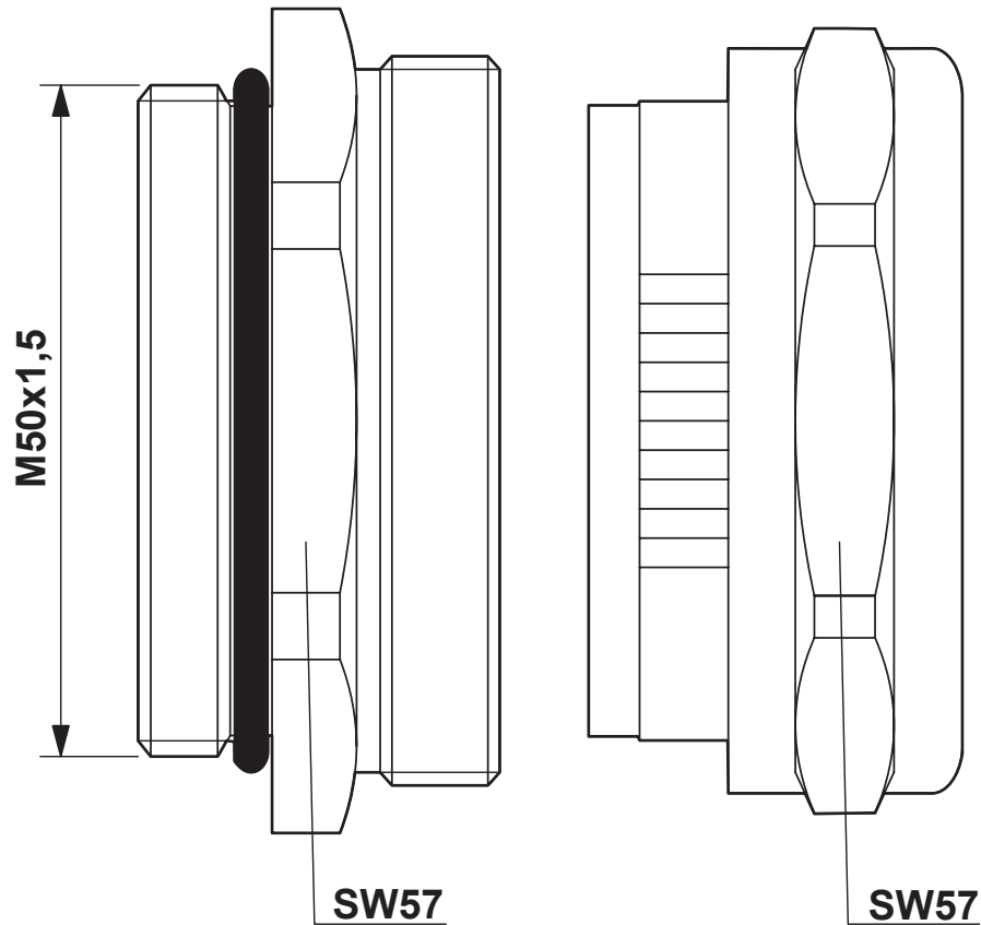
Dimensional drawing
