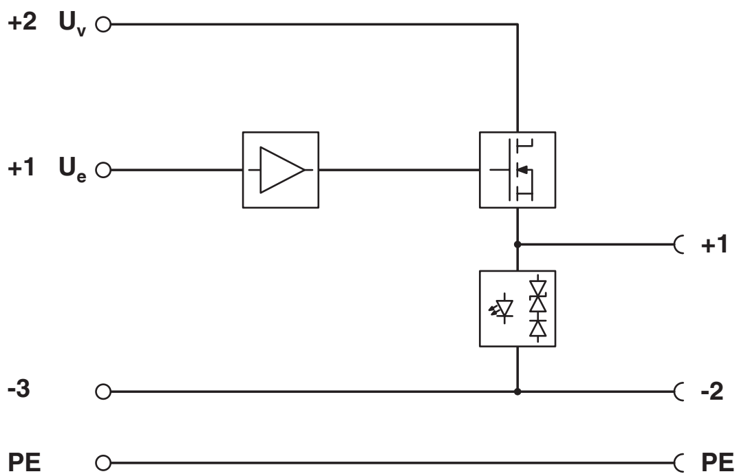
Circuit diagram
