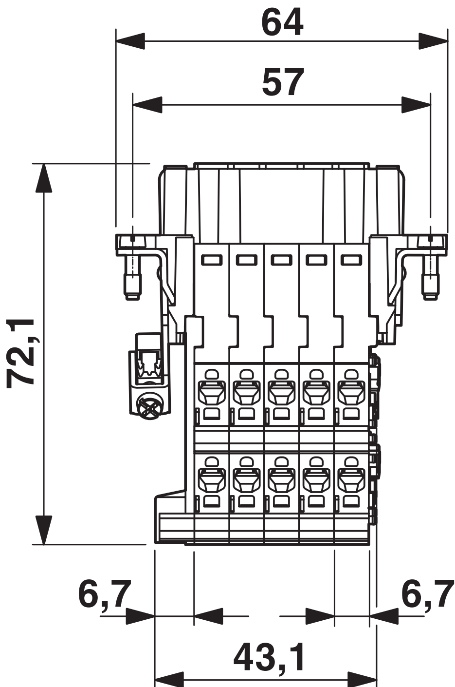
Dimensional drawing
