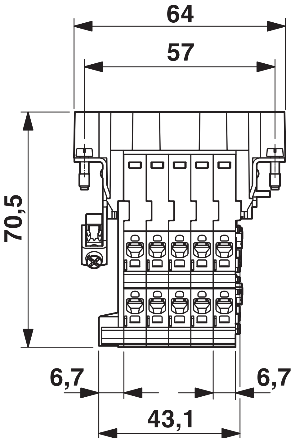
Dimensional drawing
