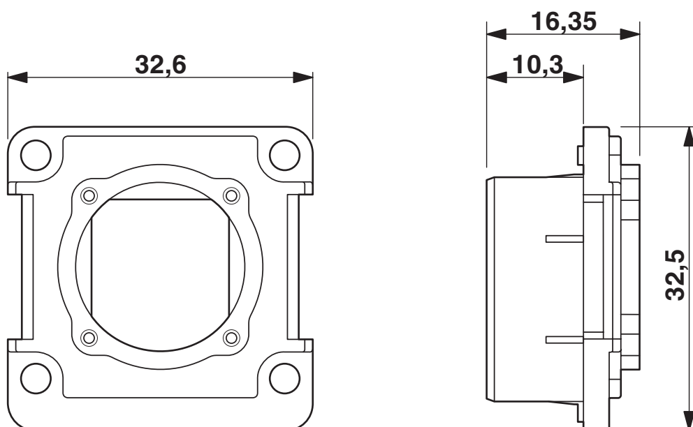
RJ45 panel mounting frame, IP67
