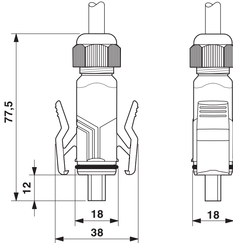
Dimensional drawing
