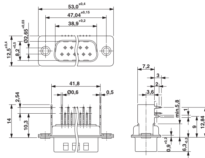
Dimensional drawing
