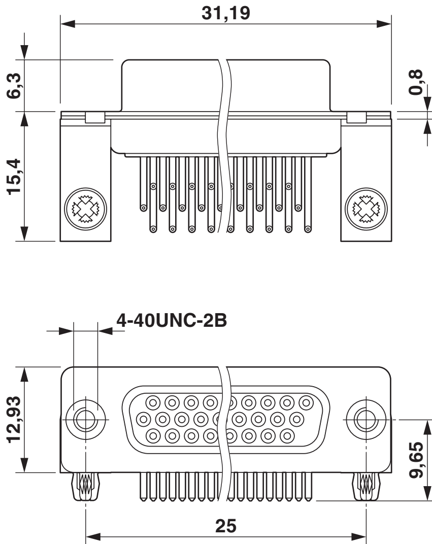
Dimensional drawing
