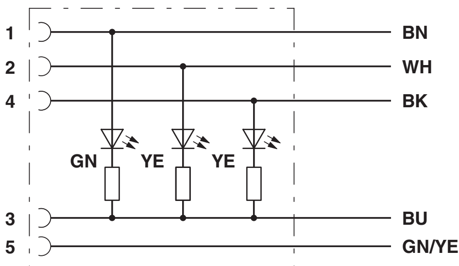
Circuit diagram
