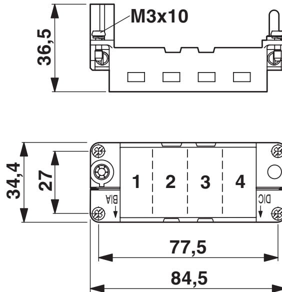
Dimensional drawing
