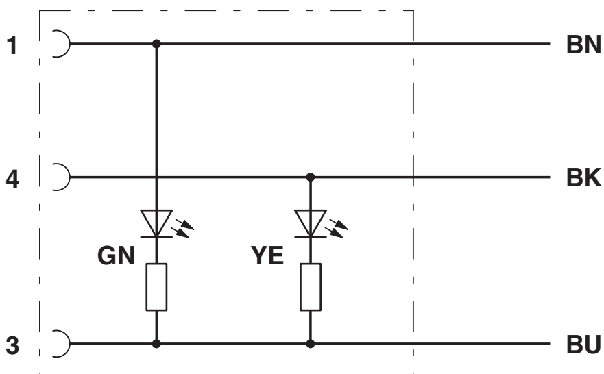
Circuit diagram
