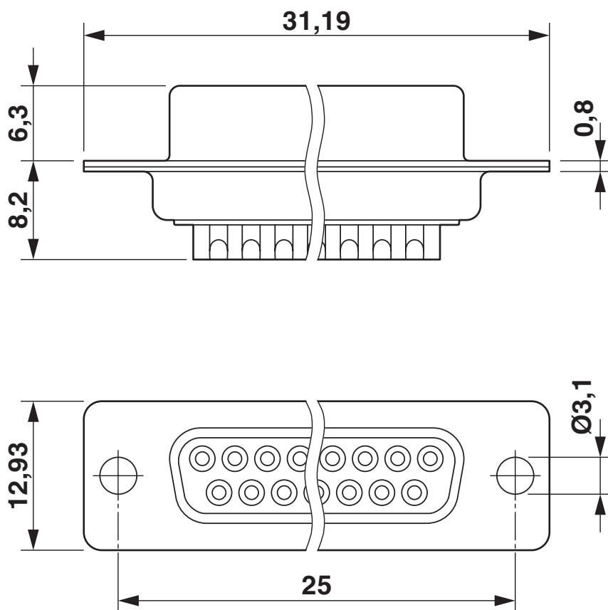
Dimensional drawing
