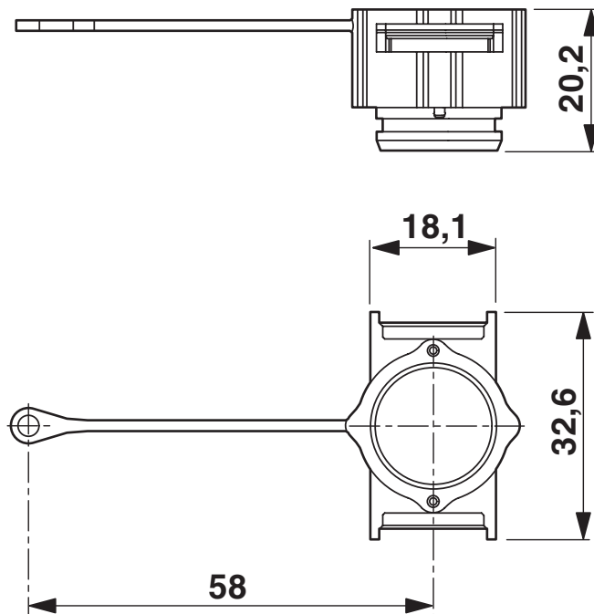
Dimensional drawing
