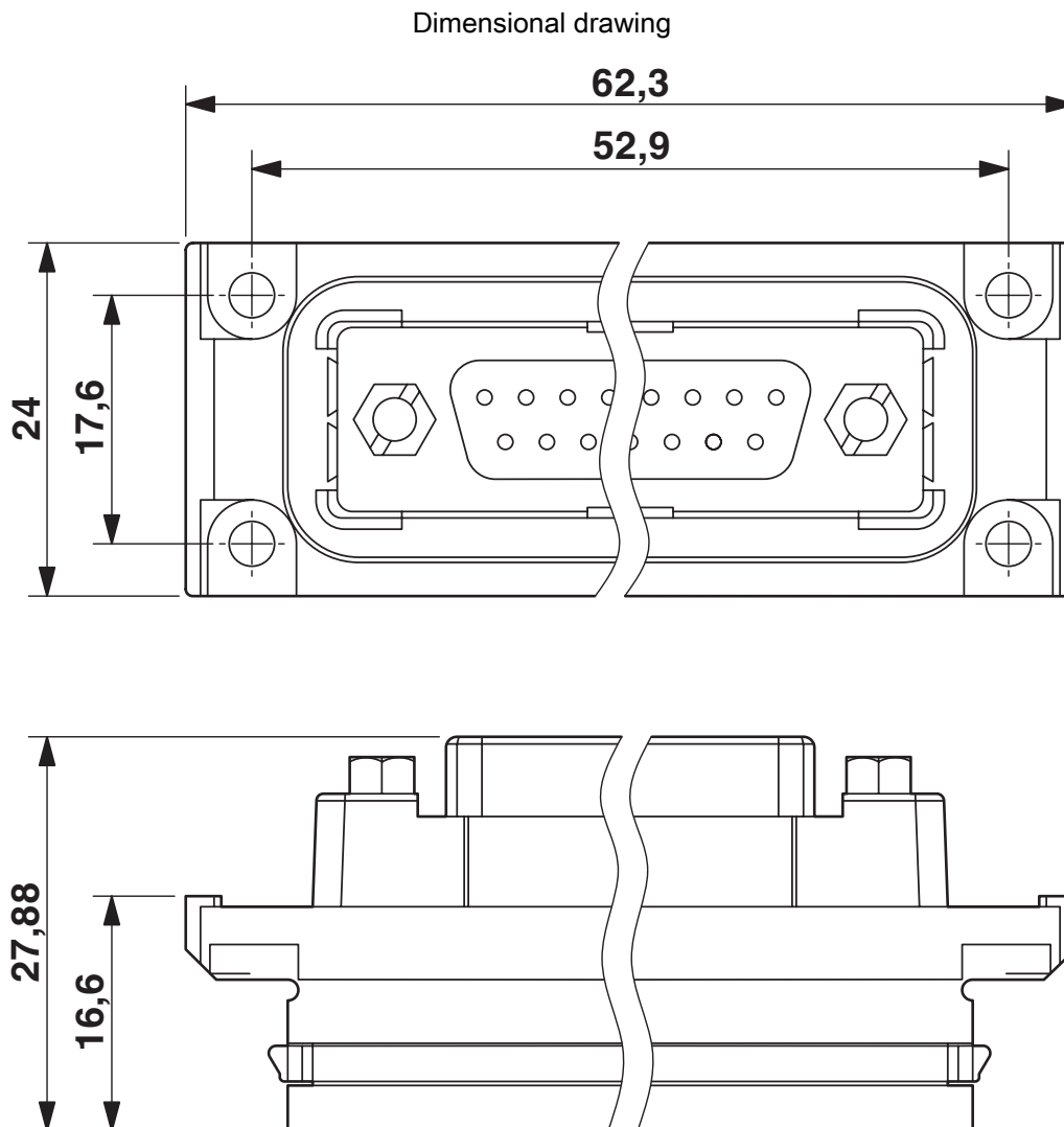
D-SUB panel mounting frame
