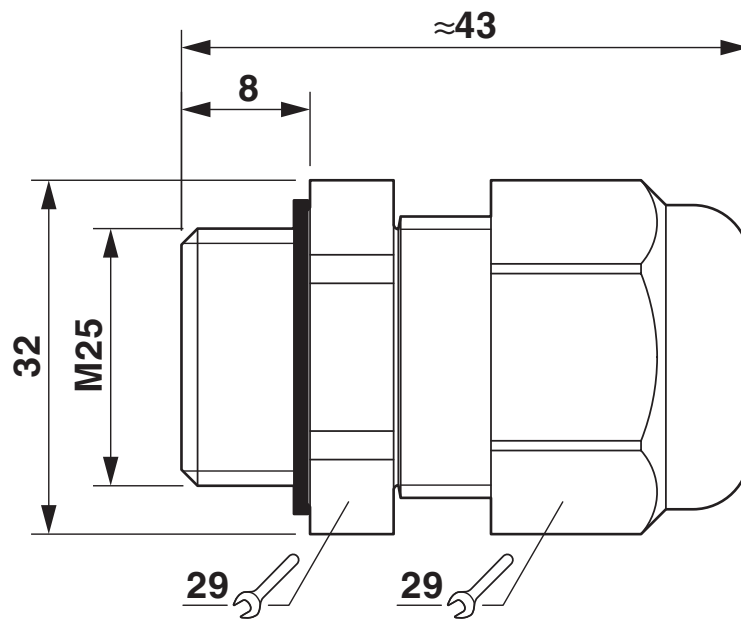
Dimensional drawing
