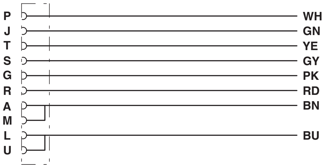
Circuit diagram
