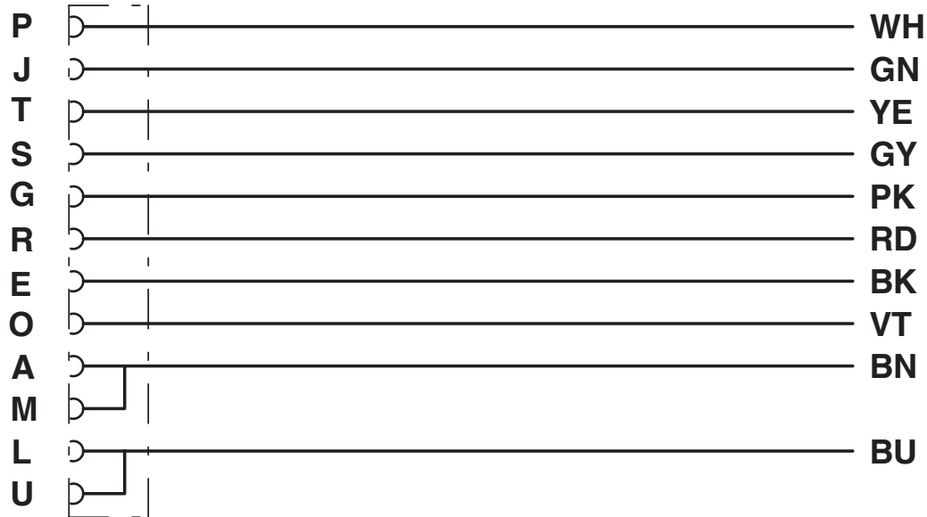
Circuit diagram
