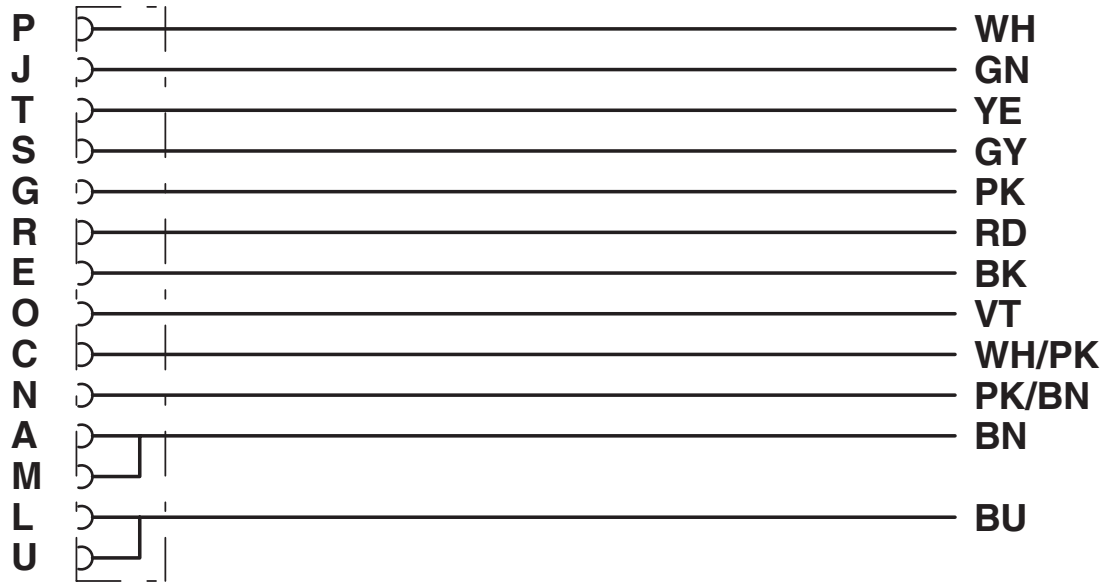
Circuit diagram
