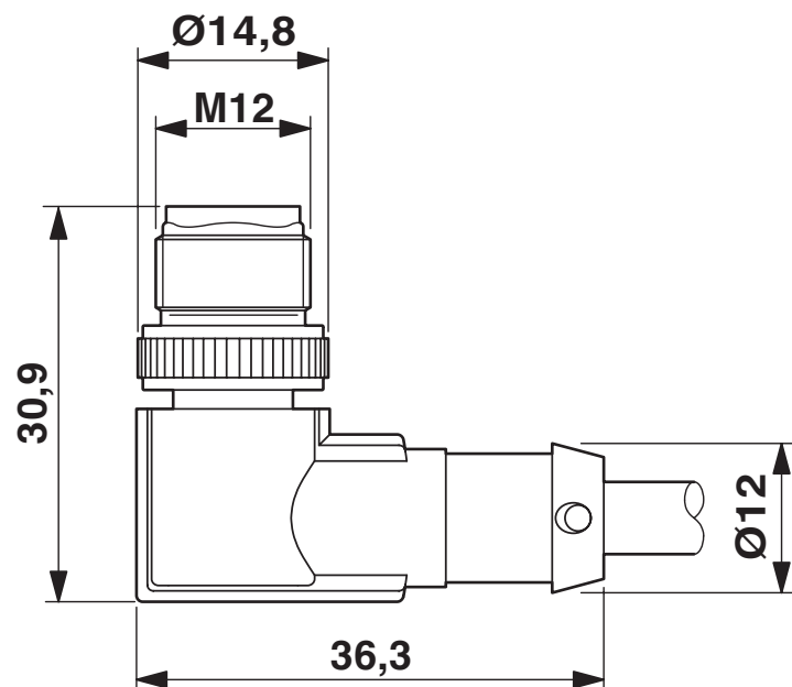
Dimensional drawing
