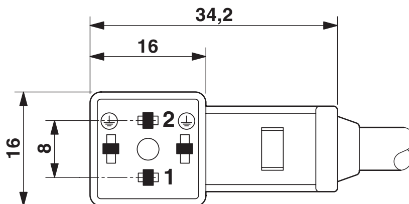
Dimensional drawing
