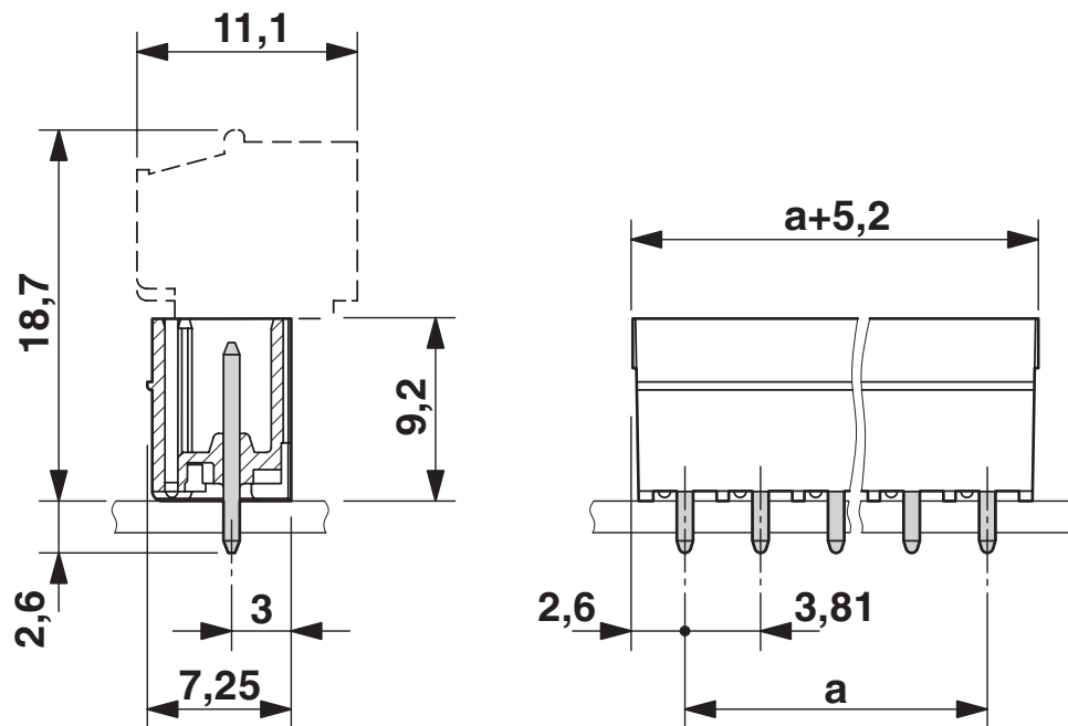
Dimensional drawing
