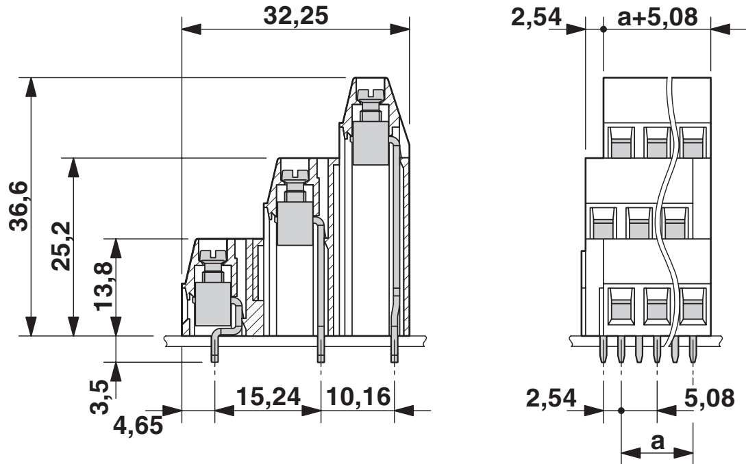
Dimensional drawing
