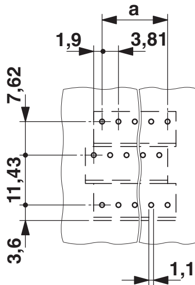
Dimensional drawing
