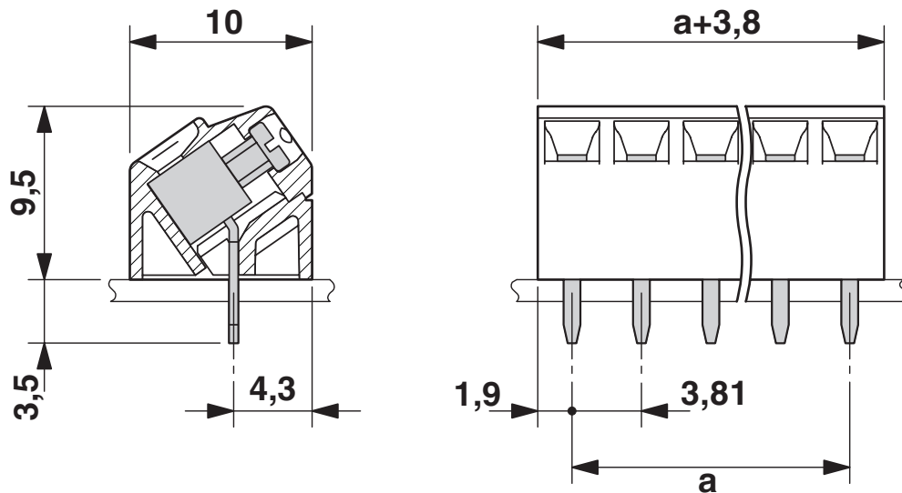
Dimensional drawing
