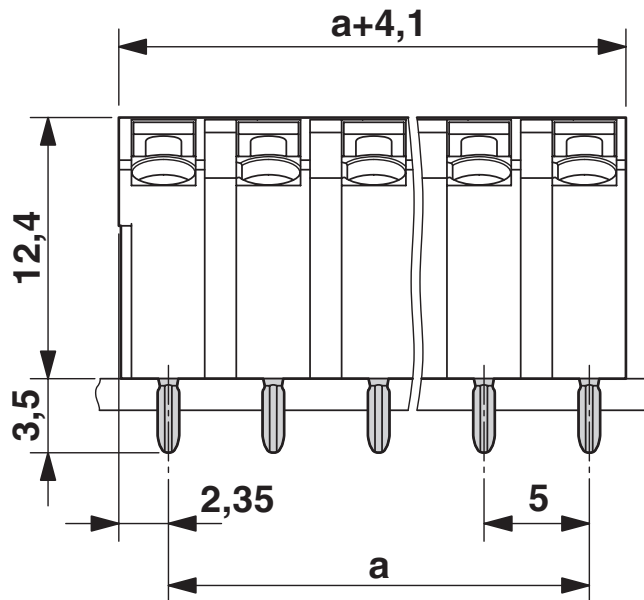
Dimensional drawing
