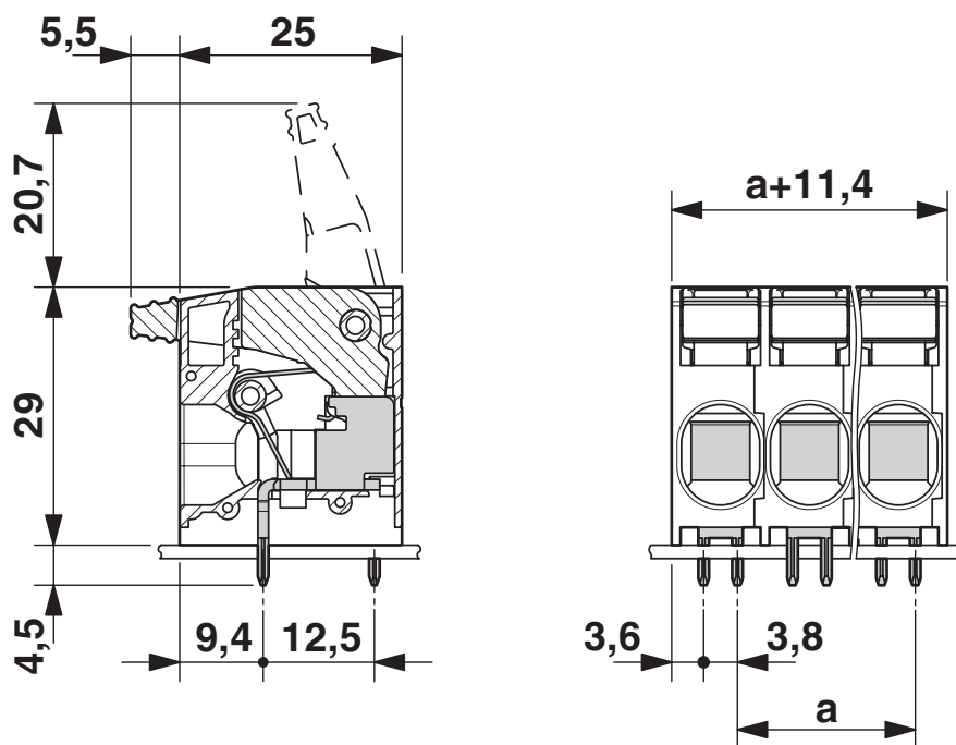
Dimensional drawing
