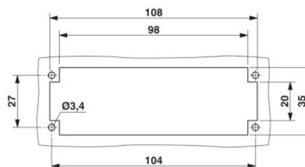
Mounting cut-out
