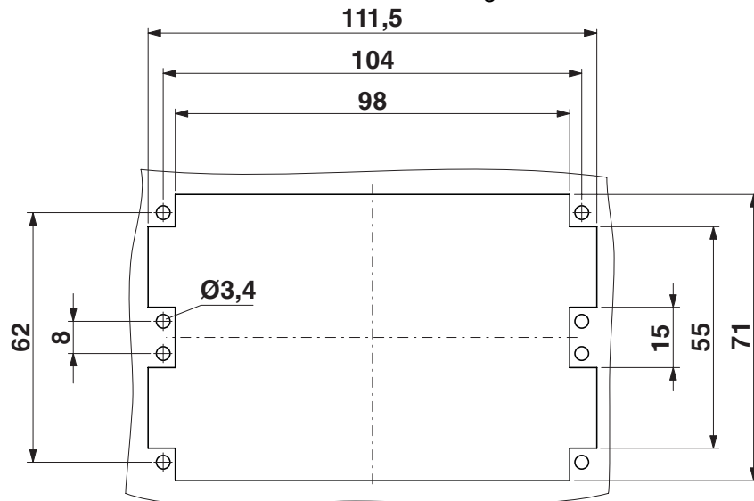
Dimensional drawing
