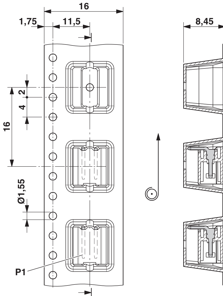
Dimensional drawing
