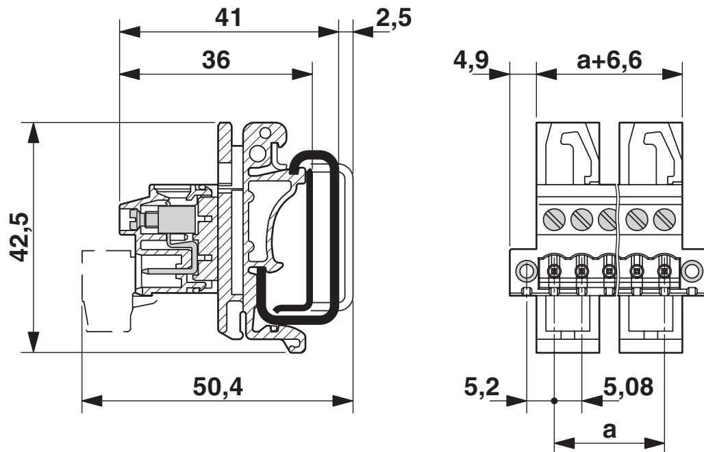
Dimensional drawing
