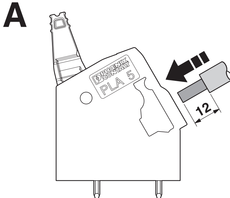
Functional drawing
