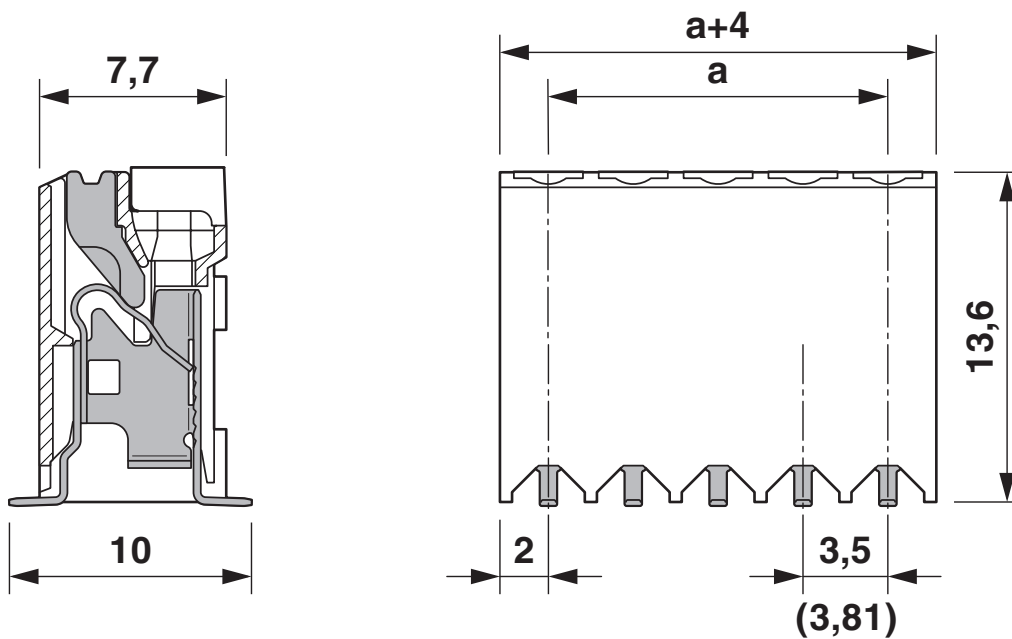
Dimensional drawing
