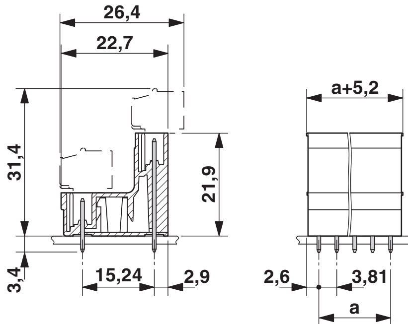
Dimensional drawing
