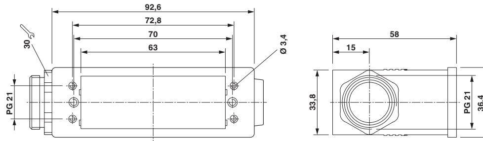
Dimensional drawing
