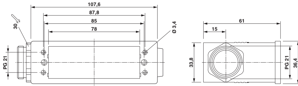
Dimensional drawing
