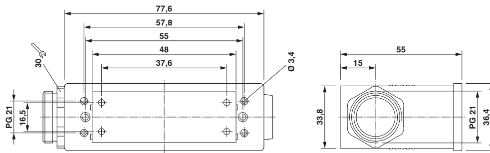
Dimensional drawing
