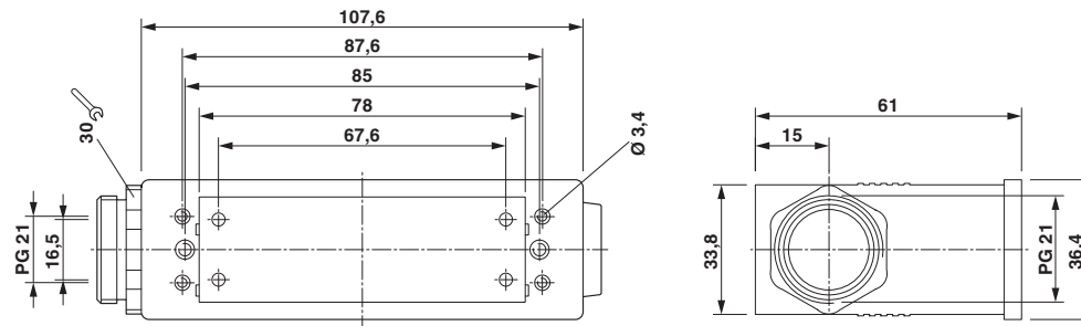
Dimensional drawing
