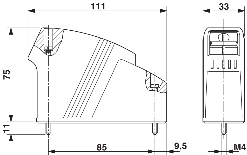
Dimensional drawing
