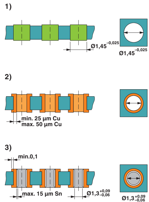
Drilling diagram
