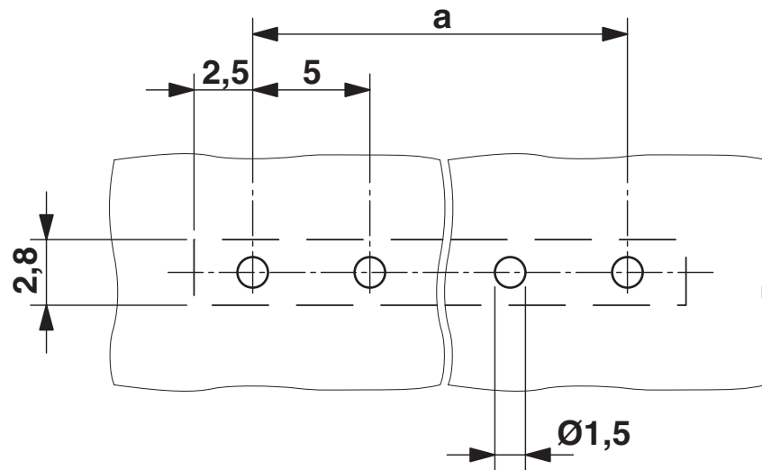
Dimensional drawing
