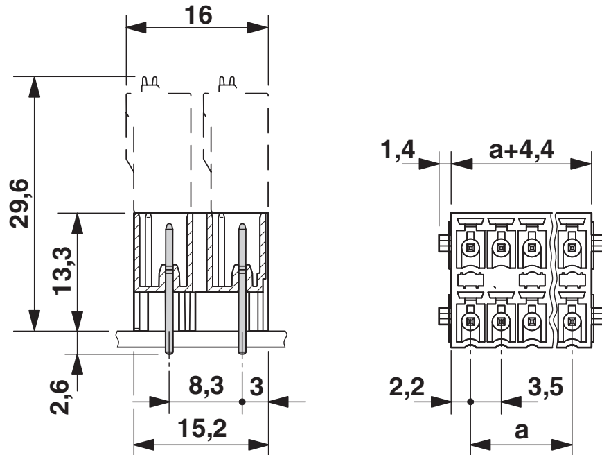
Dimensional drawing
